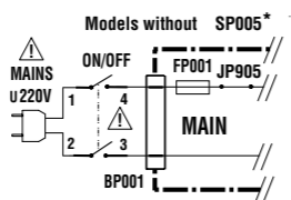
(PP) POWER SUPPLY MAIN PP 80014.00 (Stereo & Mono. without SP005 190 - 264V 25" XF & 29" XF)
